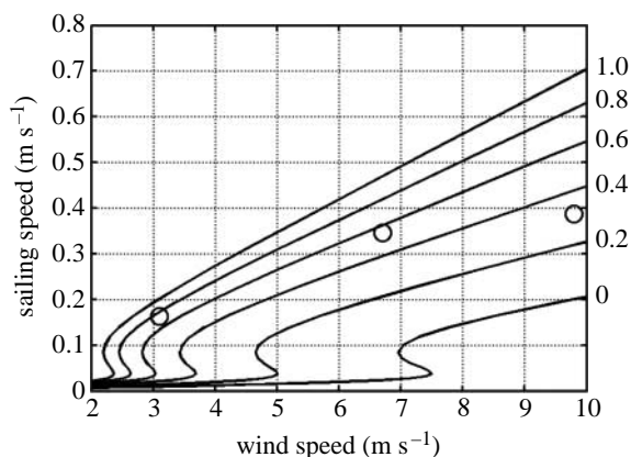
Figure 7. Sailing speed as a function of wind speed at constant side-force coefficient C_z , the value of which is marked to the right of each line. The circles are based on the observations cited in Totton & Mackie (1960).
